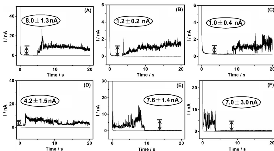
Figure 3. Chronoamperometric profiles showing catalytic oxidative Faradaic steps of N-CNT-Pd in 0.77 \text{ mM} \text{H}_2 , 0.2 \text{ M} \text{KNO}_3 at 0.1 \text{ V} (vs. \text{Ag/AgCl} ). Profiles A, B, C, and D show the collision of N-CNT-Pd with the wire electrode, while E and F show the falling off of N-CNT-Pd from the wire electrode.
